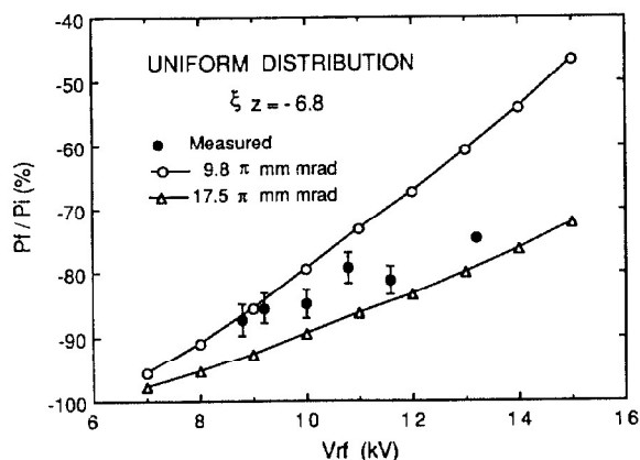
Fig. 3. Dependence of polarization ratios before and after crossing the \Upsilon G = \nu_z resonance in the booster on the rf voltage.
