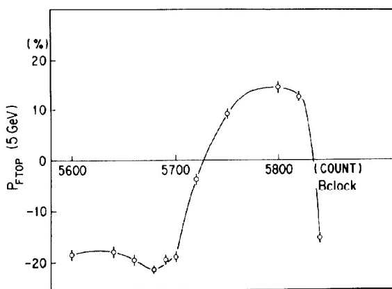
Fig. 5. Correction curve for the \Upsilon G = 4+\nu_z resonance by the slow passage method.
