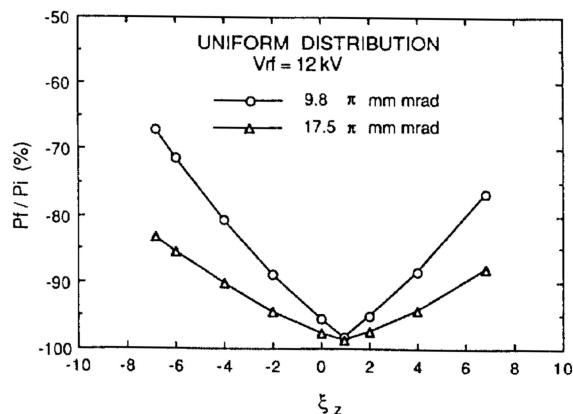
Fig. 6. Dependence of polarization ratios before and after crossing the \gamma G=\nu_z resonance in the booster on the vertical chromaticity.
