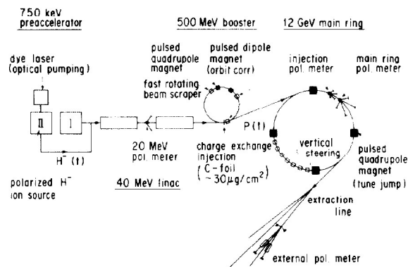
Fig. 1. Equipment designed for the polarized beam acceleration.
