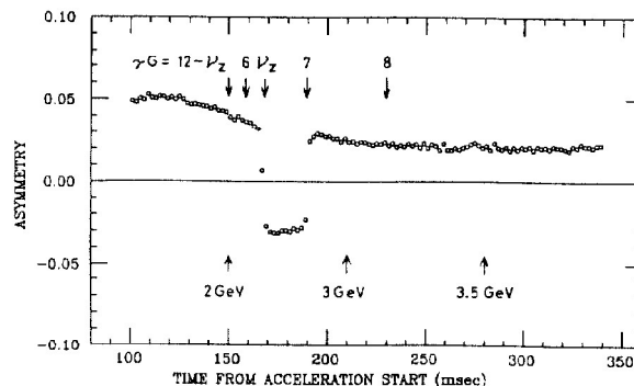
Fig. 2. The asymmetry continuously measured during acceleration.
