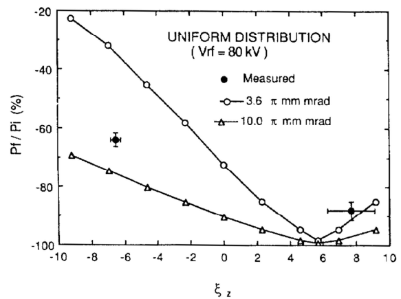
Fig. 7. Dependence of polarization ratios before and after crossing the \gamma G=\nu_z resonance in the main ring on the vertical chromaticity.
